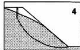
Water emits about halfway between toe and top of cut. Surface water enters upper slope cut (2 x Ht.)
