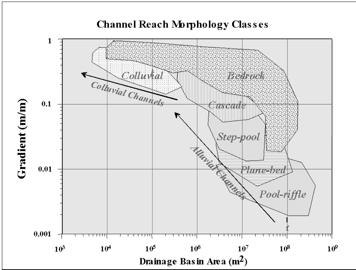
APPENDIX FIGURE II. RELATIONSHIP AMONG CHANNEL MORPHOLOGY, BASIN SIZE AND GRADIENT (adapted from Montgomery and Buffington 1997).
